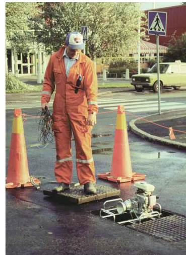
The mini-winch can be made to fit different kinds of manhole openings.
